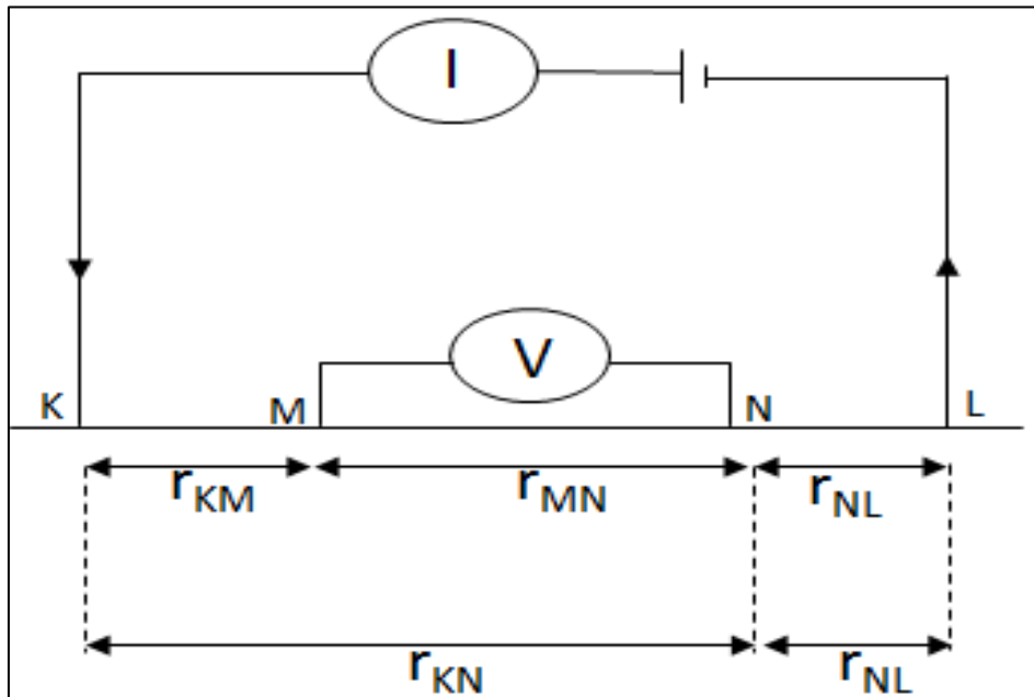
Figure-2. Diagrammatical illustration of resistivity method
