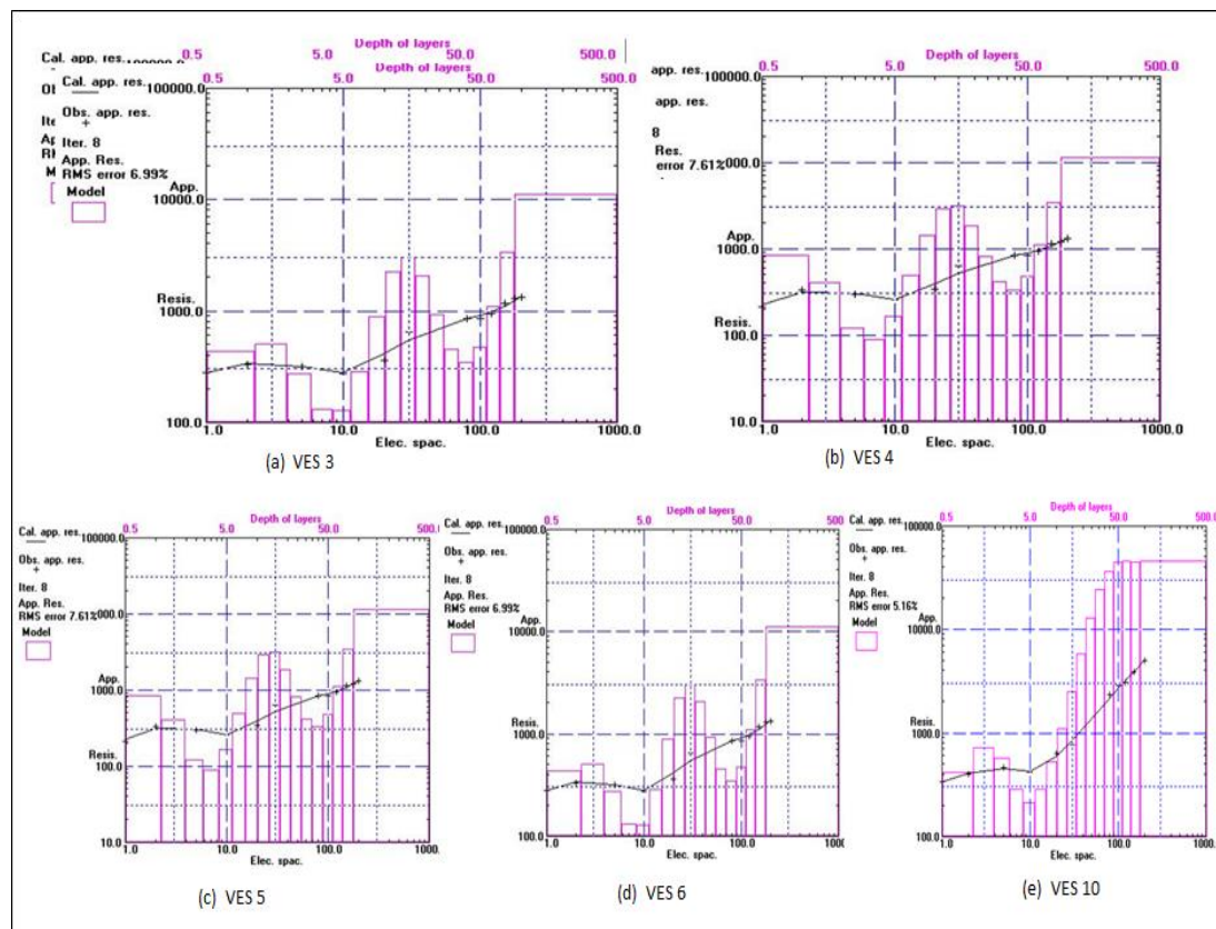
Figure-5. Inversion model for resistivity data acquired in Ehor, Edo State Nigeria
