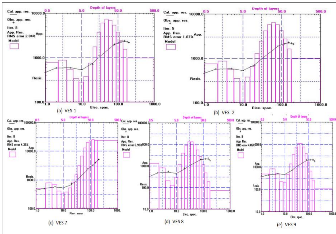
Figure-4. Inversion model for resistivity data acquired in Igeduma and adjacent vallages (Ukpho and Ukphi), Edo State
