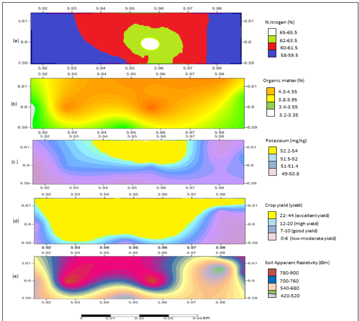
Figure-7. Comparison of spatial distribution of basic soil nutrients, soil resistivity, and crop yield in the study area
