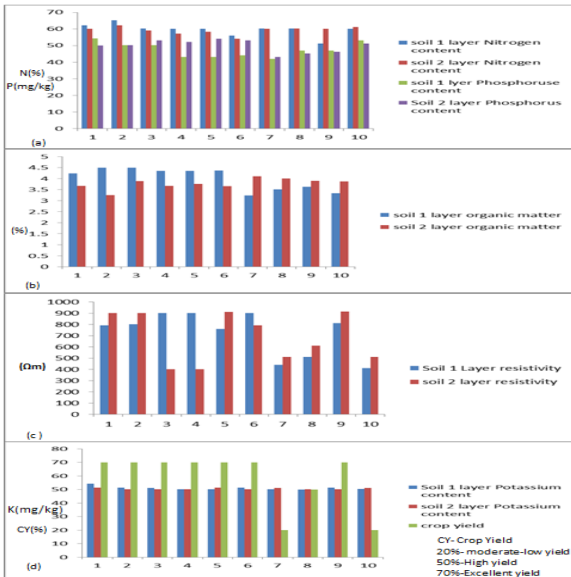
Figure-9. Descriptive statistical analyses of basic soil nutrients, soil resistivity, and crops yield in the study area
